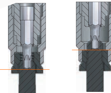
counter-holder bit in start position
